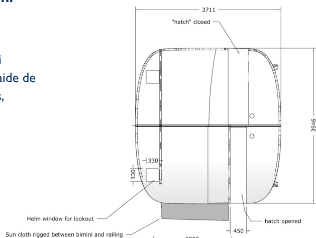
Plan 2D du Bimini carbone
